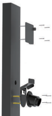
Figure 4-11 Holders Installation
