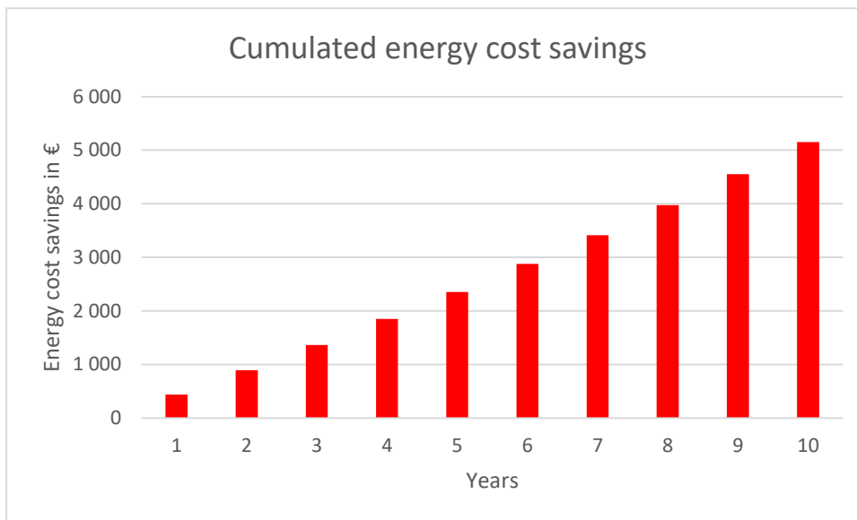
Figure 17: Cumulative energy cost savings over 10 years in €
