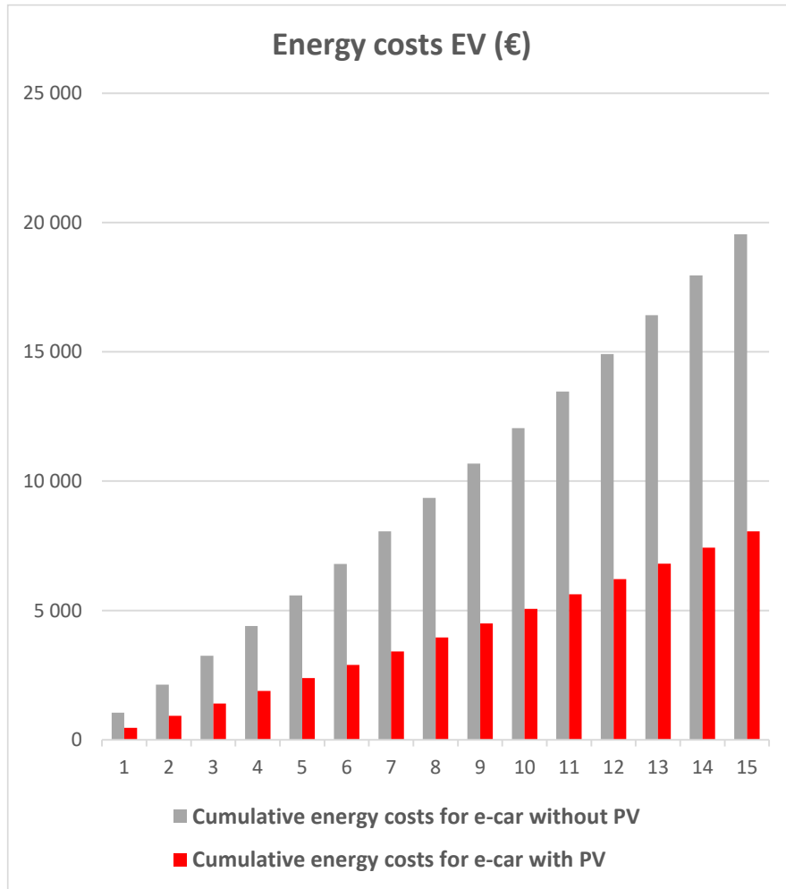
Figure 2: Cumulative energy costs for an electric car with and without PV system
