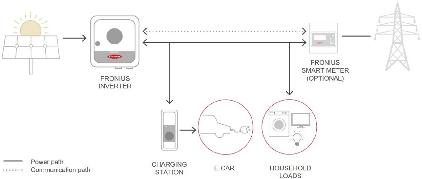
Figure 14: Configuration diagram 'manual charging with PV energy'
