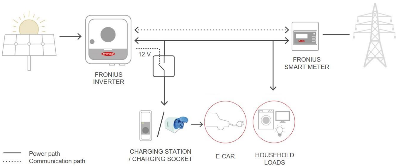
Figure 12: Configuration diagram 'Charging with inverter-integrated energy management from Fronius'
