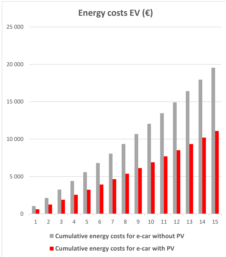
Figure 16: Cumulative energy costs for an electric car with and without PV system
