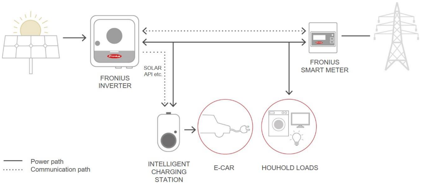
Figure 6: 'Dynamic PV surplus charging' configuration diagram
