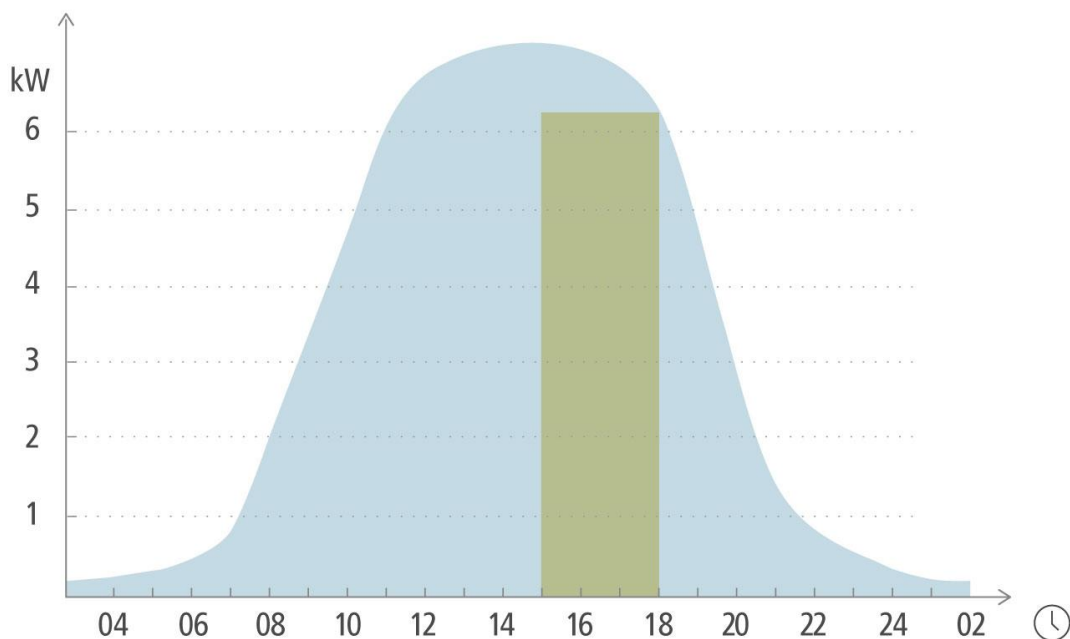
Figure 13: Functional principle of charging using inverter-integrated energy management
