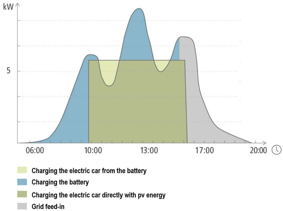
Figure 20: Charging the electric car from a battery storage
