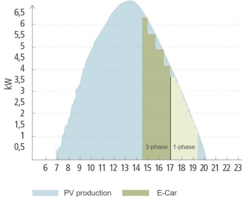
Figure 7: 'Dynamic PV surplus charging' functional principle
