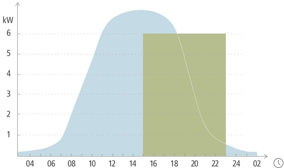
Figure 15: Functional principle of manual charging with PV energy
